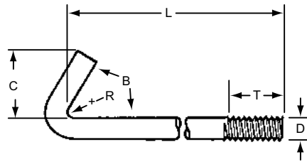
D1LA Hook Bolt, Special (L, C, A, R, B)
