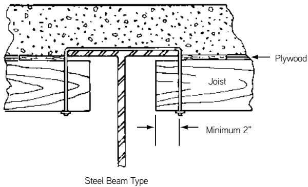
Steel Beam Type
