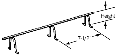
CHC Continuous High Chair CHCU-Cont. High Chair Upper
