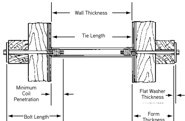
Coil Tie as Spreader and Tie
